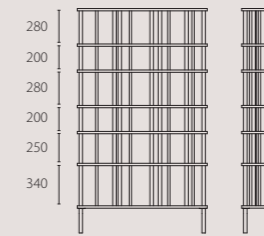
LE1106 H 1900 W 1100 D 320
