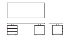
SNR4 cm. 220x90x72h. inch 86"½x35"½x28"½h.
