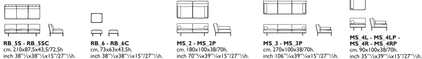
RB_5S - RB_5SC cm. 210x87,5x43,5/72,5h. inch 38 1/2x33 1/2x15 1/4/27 1/2h. RB_6 - RB_6C cm. 73x63x43,5h. inch 38 1/2x33 1/2x15 1/4/27 1/2h. MS_2 - MS_2P cm. 180x100x38/70h. inch 70 1/2x33 1/2x15 1/4/27 1/2h. MS_3 - MS_3P cm. 270x100x38/70h. inch 106 1/4x33 1/2x15 1/4/27 1/2h. MS_4L - MS_4LP - MS_4R - MS_4RP cm. 90x100x38/70h. inch 35 1/2x33 1/2x15 1/4/27 1/2h.
