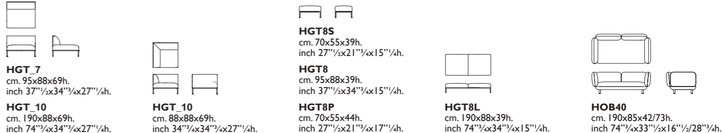
HGT_7 cm. 95x88x69h. inch 37 1/2x34 3/4x27 1/4h. HGT_8 cm. 95x88x39h. inch 37 1/2x34 3/4x15 1/4h. HGT8P cm. 70x55x44h. inch 27 1/2x21 3/4x17 1/4h. HGT8L cm. 190x88x39h. inch 74 1/2x34 3/4x15 1/4h. HGT10 cm. 88x88x69h. inch 34 3/4x34 3/4x27 1/4h. HOB40 cm. 190x85x42/73h. inch 74 1/2x33 1/2x16 1/2/28 3/4h.
