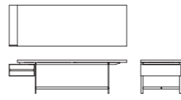
LH_8L cm. 258x90x73h. inch 101"½x35"½x28"½h.
