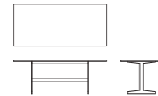
S8_T1 cm. 220x90x72h. inch 86"½x35"½x28"½h.
