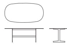
S8_T2 cm. 200x100x72h. inch 78"½x39"½x28"½h.
