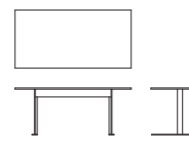
LX_1 cm. 180x90x73h. inch 70"½x35"½x28"½h.
