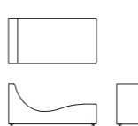
TSA3 cm. 135x70x28/41/72h. inch 53 1/8x27 1/8x11 1/8/16 1/4/28 3/4h.
