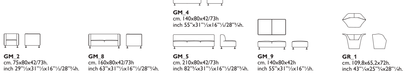
GM_2 cm. 75x80x42/73h. inch 29 1/2x31 1/2x16 1/2/28 3/4h. GM_8 cm. 160x80x42/73h. inch 63 1/2x31 1/2x16 1/2/28 3/4h. GM_5 cm. 210x80x42/73h. inch 82 1/2x31 1/2x16 1/2/28 3/4h. GM_9 cm. 140x80x42h. inch 55 1/2x31 1/2x16 1/2h. GM_4 cm. 140x80x42/73h. inch 55 1/2x31 1/2x16 1/2/28 3/4h. GR_1 cm. 109x8x65,2x72h. inch 43 1/2x25 1/2x28 1/4h.
